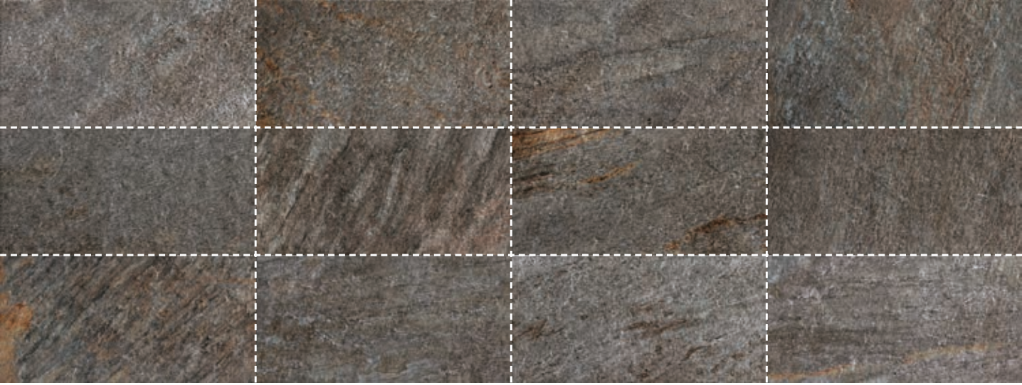
mantle_05
