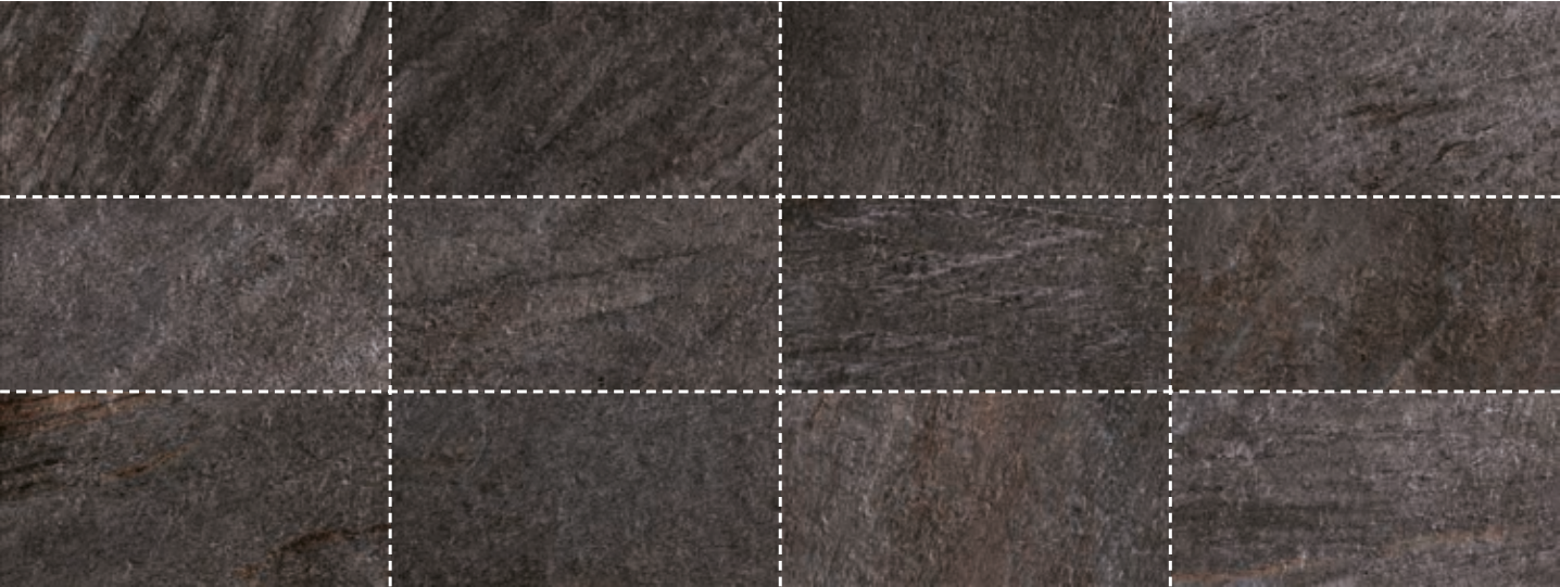
mantle_05
